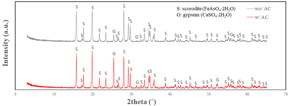
Fig. 5. XRD analysis of iron-arsenic precipitation from the oxidative reactions with/without activated carbon injecting air.
