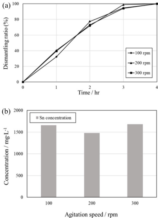
Fig. 3. The effects of agitation speed on the (a) dismantling of components and (b) leaching of Sn from PCB.
