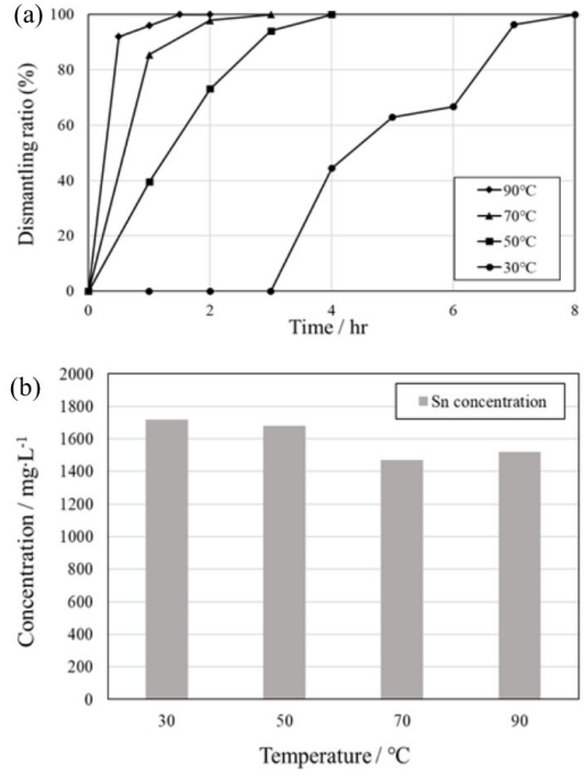
Fig. 4. The effects of temperature on the (a) dismantling of components and (b) leaching of Sn from PCB.
